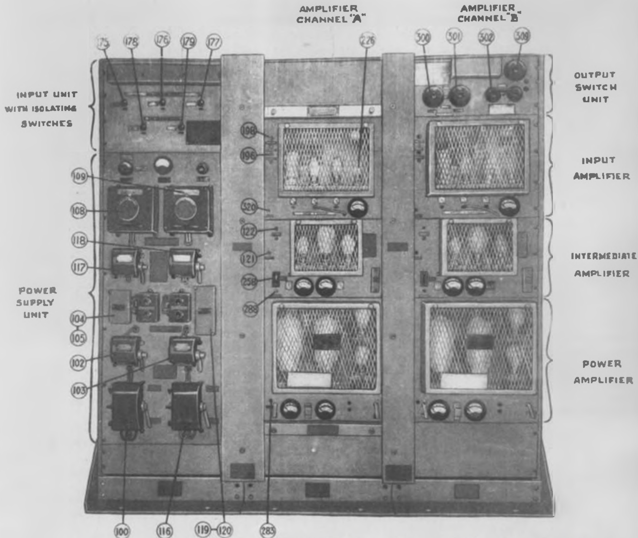
Type 405 main gear. Half the size of the Type 401
