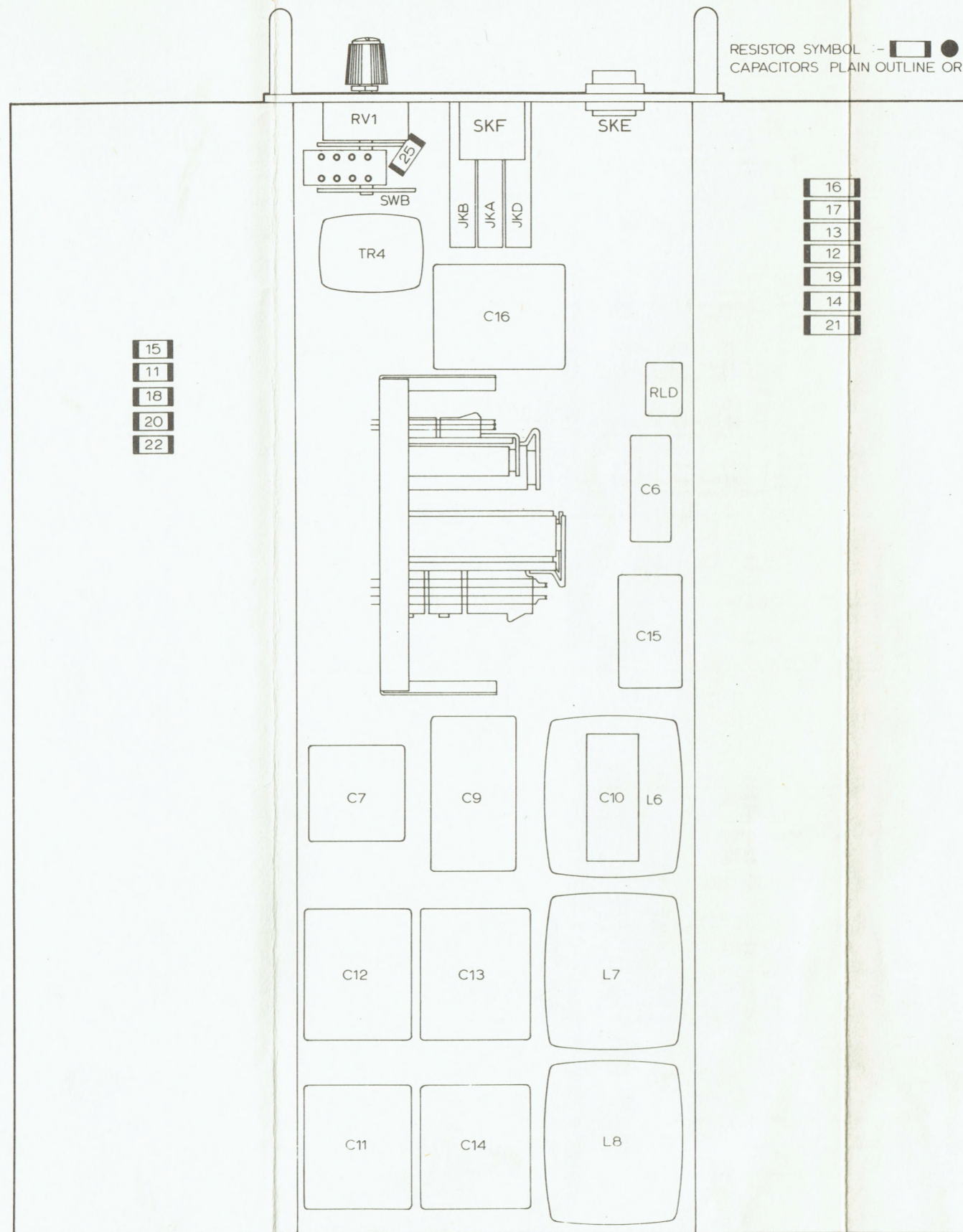
POWER SUPPLY UNIT CHASSIS 2 COMPONENT LAYOUT DIAGRAM AP100340 OR AP399015
