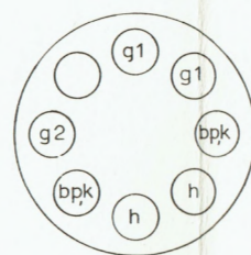
CV428 5B/251M
