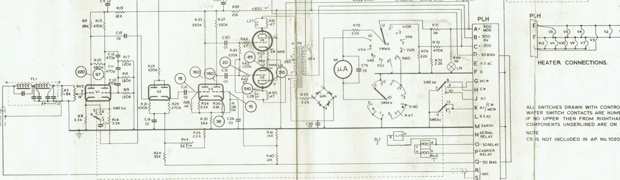
H.F. TRANSMITTER CIRCUIT DIAGRAM AP100337
