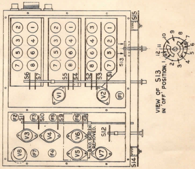
Fig. 7. Position of Switches.
