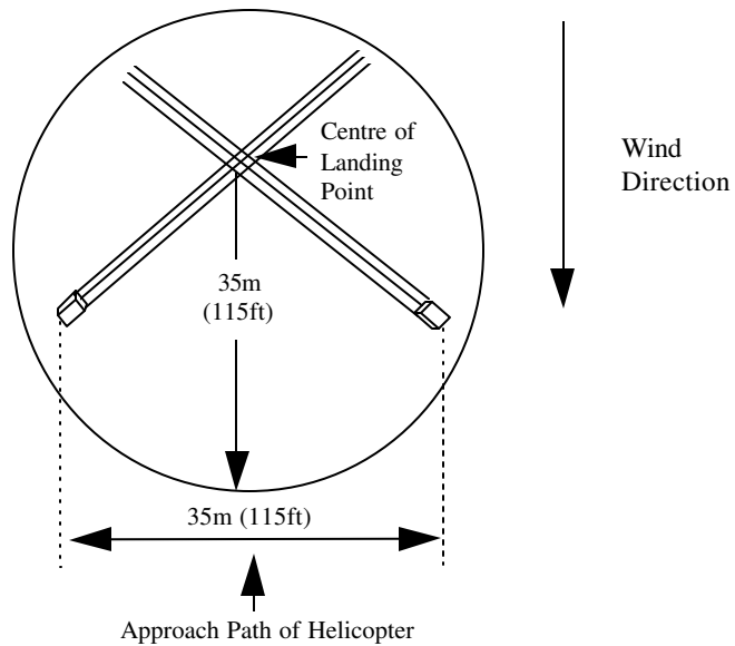
Figure 10-6 Visual Marking Of Helicopter Landing Site By Night
