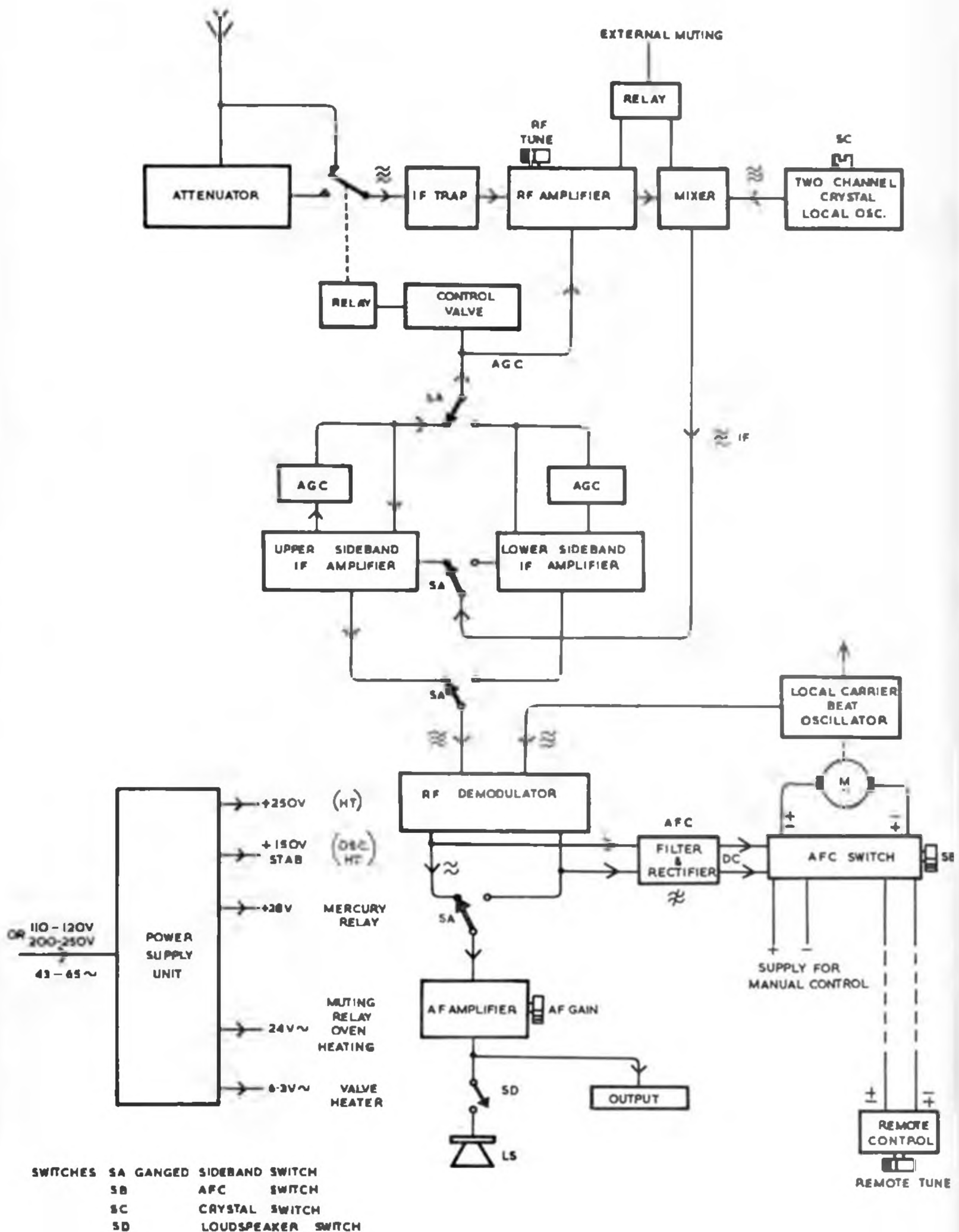
RECEIVER BLOCK DIAGRAM
