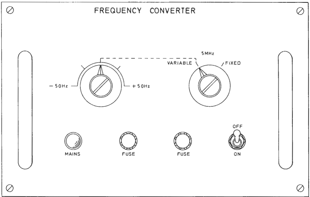
FRONT PANEL
