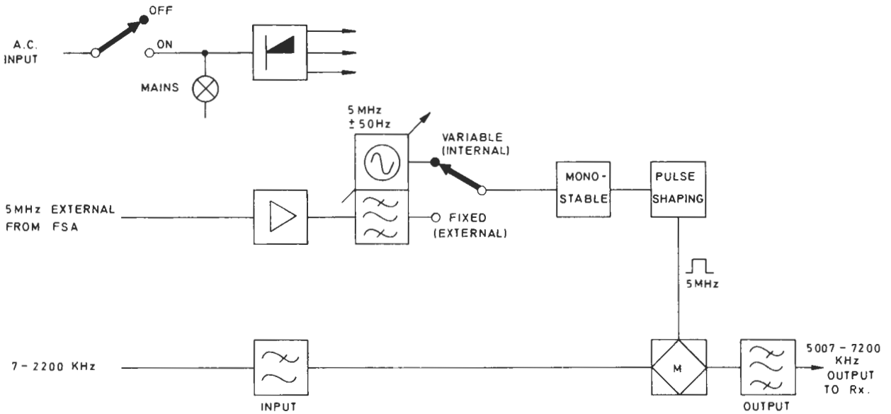
BLOCK DIAGRAM
