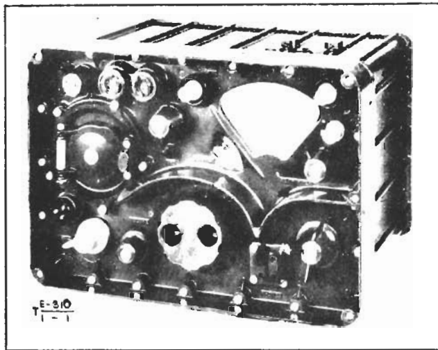
Fig. 1 Front view of equipment
