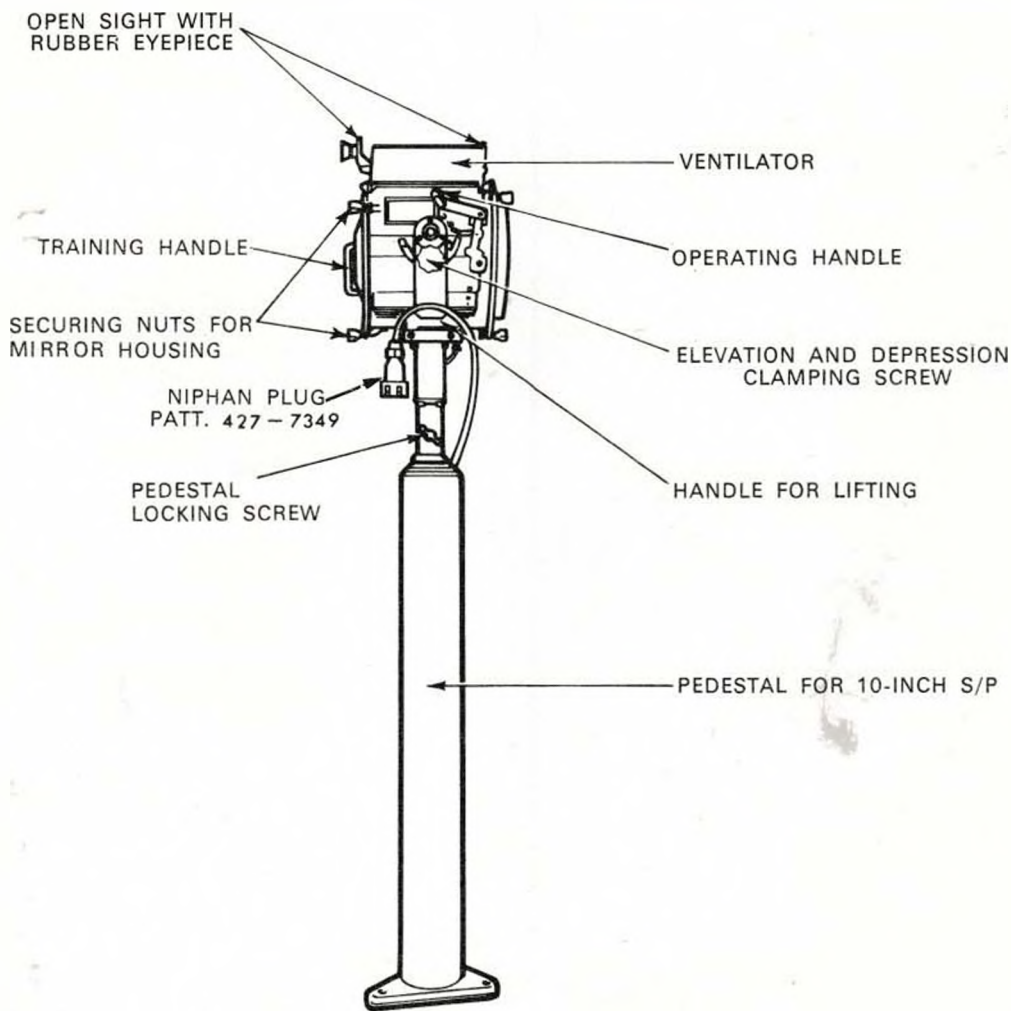
10 - INCH SIGNALLING PROJECTOR LIGHT - FIG. 3,3
