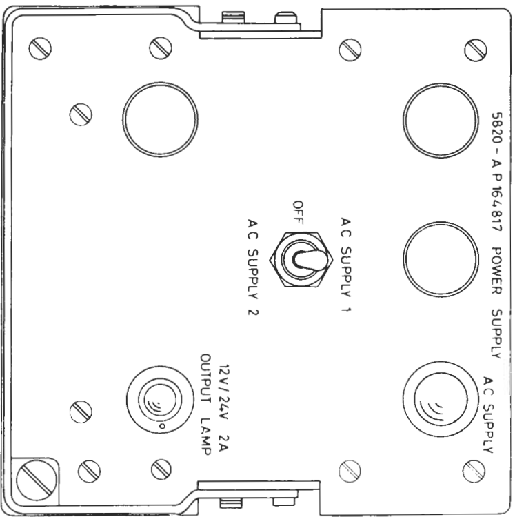
j POWER SUPPLY UNIT
