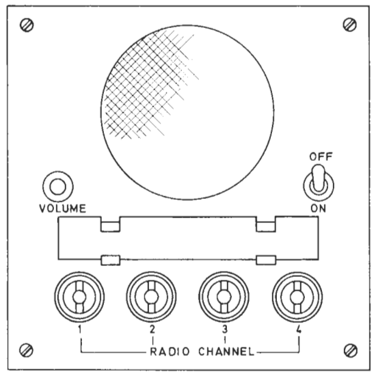
(b) VCS UNIT TYPE 102 RADIO LOUDSPEAKER 4 WAY
